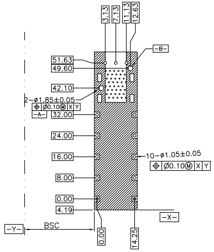
CONNECTOR PIN-OUT COMPONENT SIDE OF BOARD
