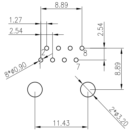
PCB LAYOUT TOP VIEW DIMENSIONS TOLERANCE:±0.05
