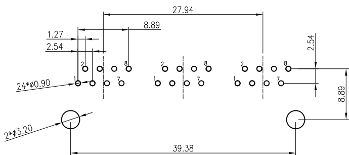
PCB LAYOUT TOP VIEW DIMENSIONS TOLERANCE:±0.05
