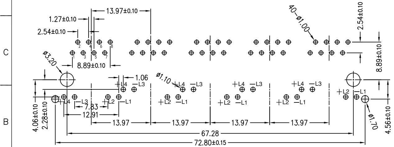
RECOMMENDED P.C.B. LAYOUT TOP VIEW (俯视图)
